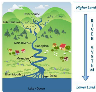
Features of a River
